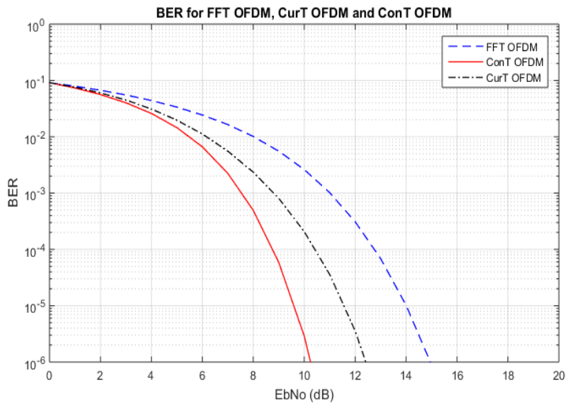
Figure 11. BER for the considered systems using 8 PSK
