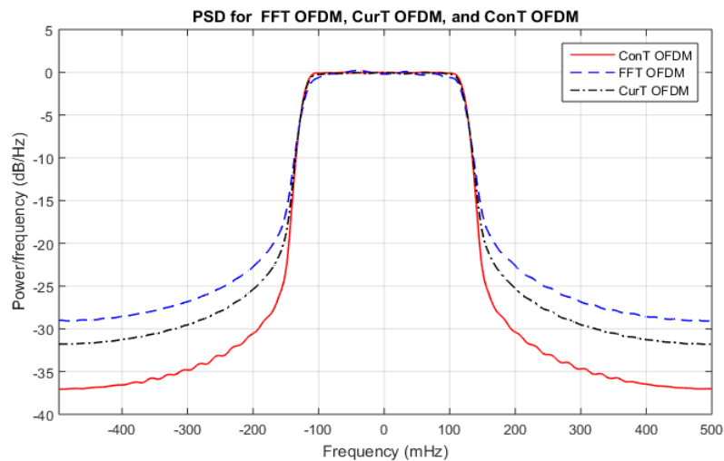
Figure 13. PSD for the considered systems using 64 subcarriers
